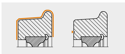
Wheels
